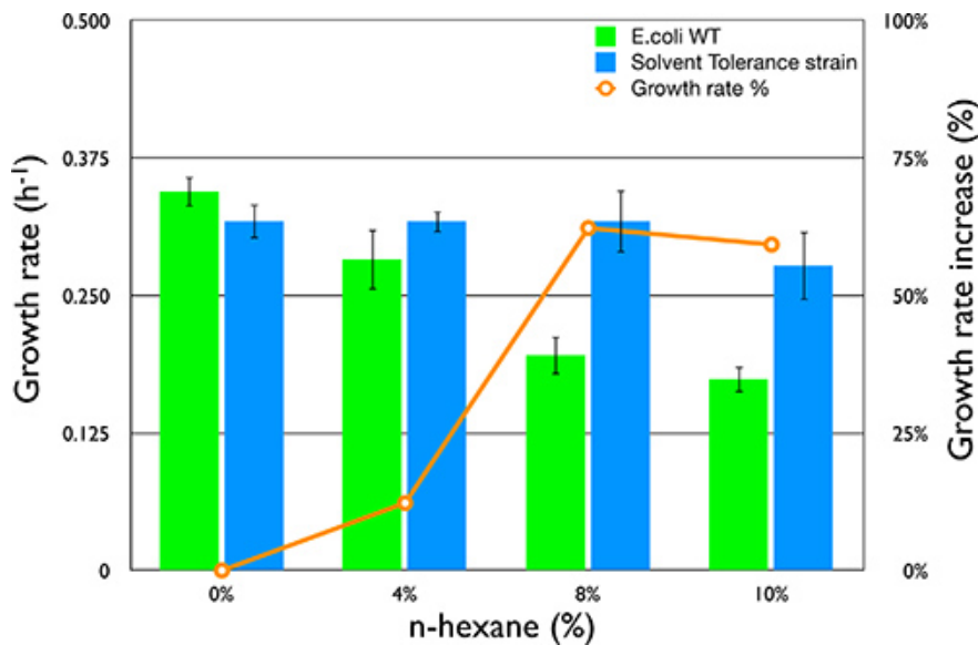
Figure 5. Solvent tolerance. The growth rate (OD 600 ) was measured of E. coli strains with a periodicity of 10 minutes. E. coli K12 expressing the solvent tolerance cluster (BBa_K398406) was tested by different amounts of n -hexane (0, 4, 8, 10%). As a control, E. coli expressing BBa_J13002-ladA was used. Error bars represent the SEM of three independent experiments.
