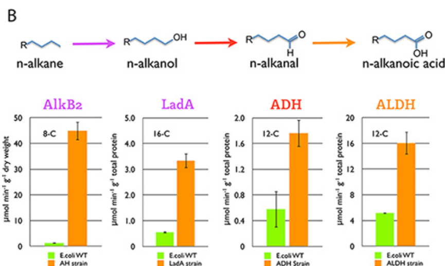
Figure 2. A three-step pathway for alkane oxidation was implemented in E. coli . (A) Flow chart of the implemented genes. Four genes ( alkB2 , rubA3 , rubA4 and rubB ) of the alkane hydroxylase (AH) system of Gordonia sp. TF6 were used to facilitate the oxidation of the medium chain alkanes to their respective alkanols. The ladA gene from Geobacillus thermodenitrificans was implemented for the conversion of long-chain alkanes. To improve the degradation process for the alcohols or aldehydes, respectively ADH and ALDH genes (alcohol and aldehyde dehydrogenase) were expressed in E. coli . The resulting alkanolic-acids were metabolized via the host's \beta -oxidation pathway. (B) Enzyme activities of alkane conversion proteins for medium- and long-chain alkanes. The biotransformation of n -octane was monitored using resting cells assays in E. coli K12 carrying the BBa_K398014 plasmid, the BBa_K398017 plasmid, the BBa_K398018 plasmid, the BBa_K398030 plasmid or control plasmid BBa_J13002 . The enzyme activities of ADH and ALDH were tested in cell extracts in vitro by monitoring the reduction of NAD to NADH. Error bars represent the SEM of three independent experiments. Click here to view larger figure.
