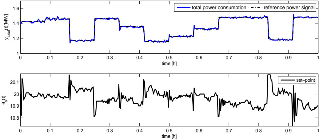
Fig. 6. Tracking of a piecewise-constant reference signal (top panel) by set-point control (bottom panel) in a homogeneous population of TCLs abstracted by the formal probabilistic approach.
