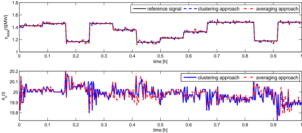
Fig. 7. Heterogeneous population of TCLs with C \in \mathcal{U}([2, 18]) : tracking of a piecewise-constant reference signal (top) by set-point control (bottom), abstracted via clustering (5 clusters) and averaging.
