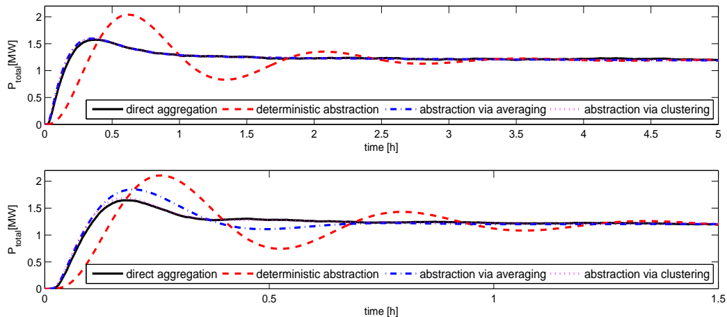
Fig. 5. Heterogeneous population of TCLs. Comparison of the deterministic abstraction from [22] with the formal probabilistic abstraction based on averaging, for two different ranges of the thermal capacitance: [8, 12] (top panel) and [2, 18] (bottom panel).
