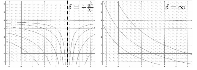
Fig. 1. The phase space of the diagonal system given in Example 1 for c = 1 (left) and c = -1 (right).
